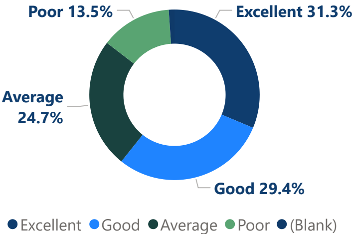
Performance Distribution
